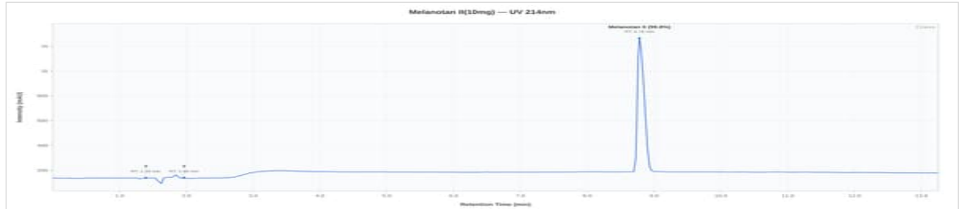
Melanotan II 10mg - MT2-2026-001: UV Chromatogram
